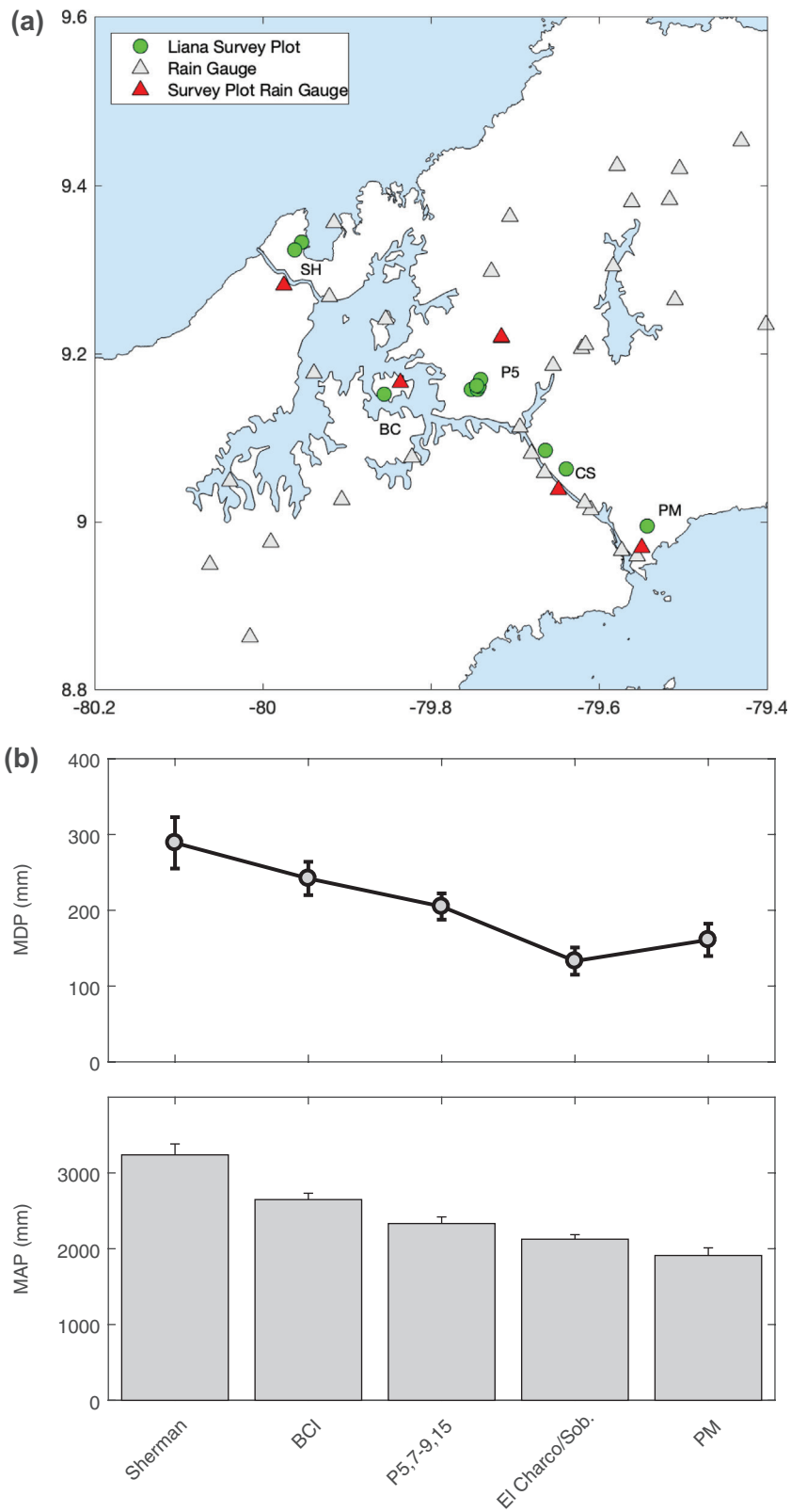
Figure 1. Isthmus of Panama precipitation gradient. (a) Locations of liana survey plots and rain gauges. Green circles indicate the eleven liana survey plots, open triangles indicate all rain gauges, and red triangles indicate rain gauges nearest to the liana survey plots. (b) Mean annual precipitation (MAP) and mean dry season precipitation (MDP) at the liana survey plots.
