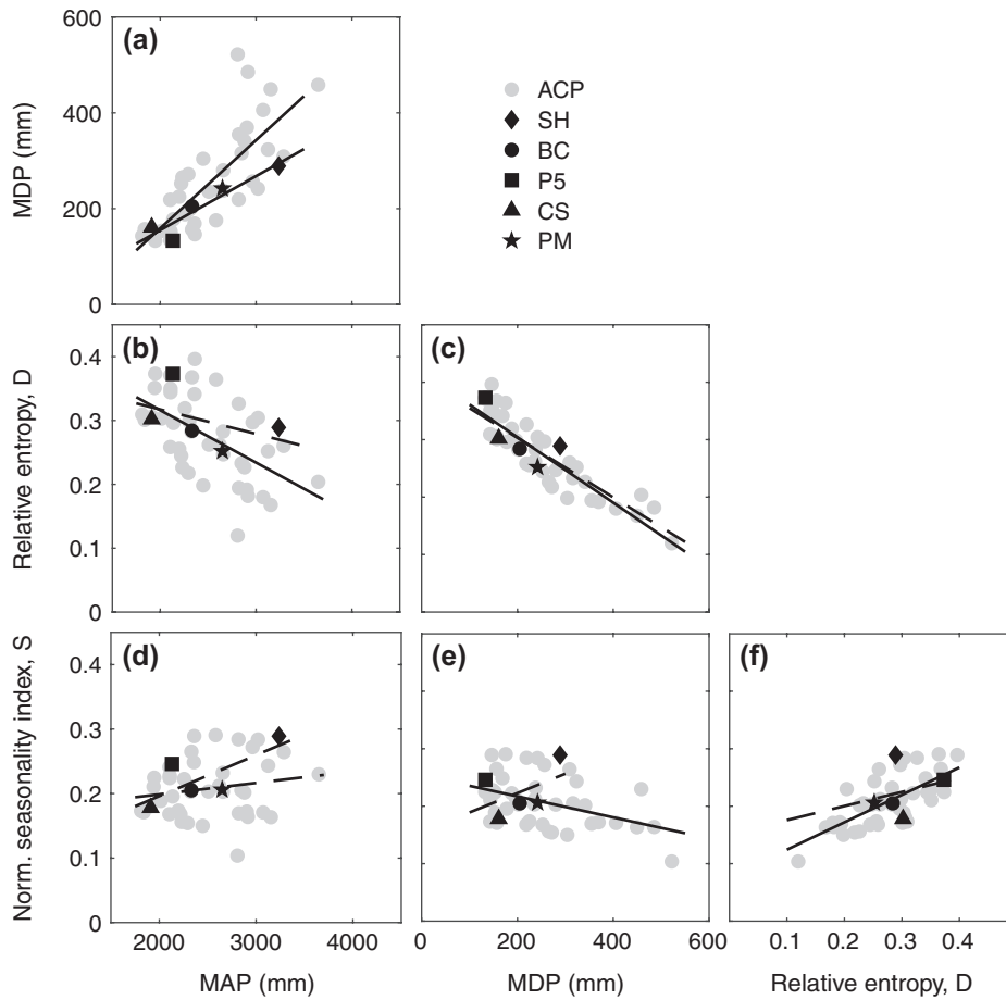
Figure 2. Seasonal and annual-scale rainfall variability across the Isthmus of Panama. Rainfall descriptors include: mean annual precipitation (MAP), mean dry season precipitation (MDP), relative entropy ( D ), and normalized seasonality index ( S ). The black symbols correspond to the five rain gauges near the liana survey plots and the gray circles correspond to 29 additional rain gauges in the study area. Lines correspond to least squares linear regressions with solid lines indicating significance with p < 0.05 . Regression parameters are listed in Supplementary material Appendix 1 Table A1. Different shaped symbols represent different sites: Sherman ( \blacklozenge ), Barro Colorado Island ( \blackstar ), Parcelas 5.7–9.15 ( \bullet ), El Charco y Soberania ( \blacksquare ), and Parque Metropolitano ( \blacktriangle ).
