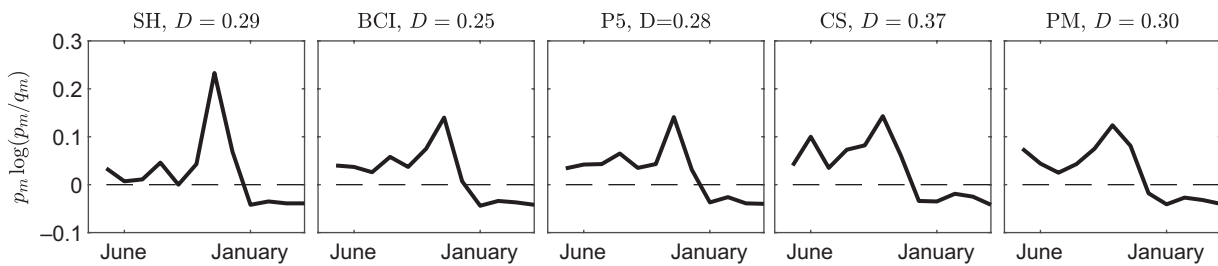
Figure 3. Monthly contributions to the relative entropy, D , for the rain gauges near the five liana survey plots. From left to right, Sherman (SH), Barro Colorado Island (BCI), Parcelas 5.7–9.15 (P5), El Charco y Soberania (CS) and Parque Metropolitano (PM).
